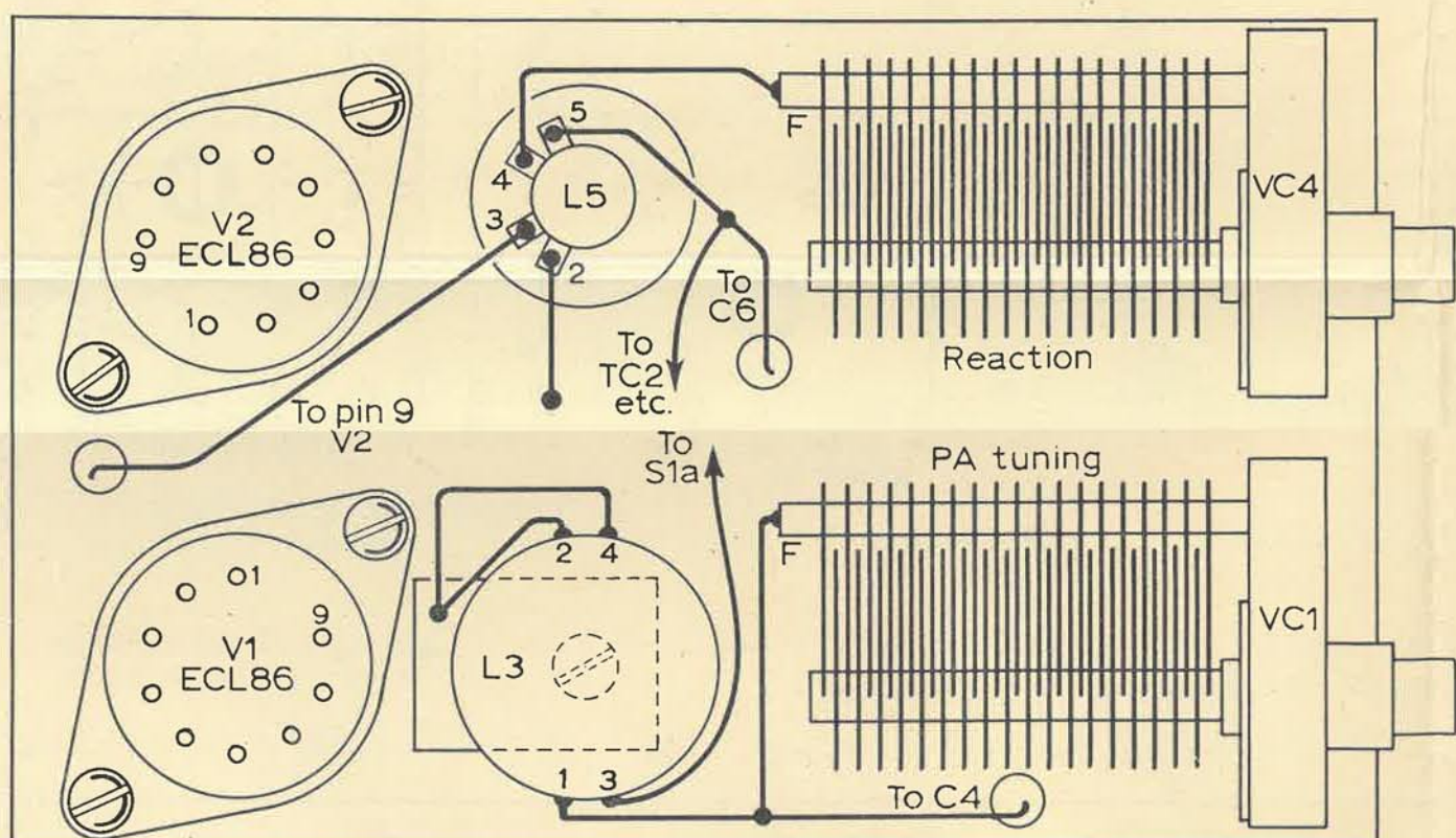
FIG. 2 TOP VIEW OF CHASSIS
