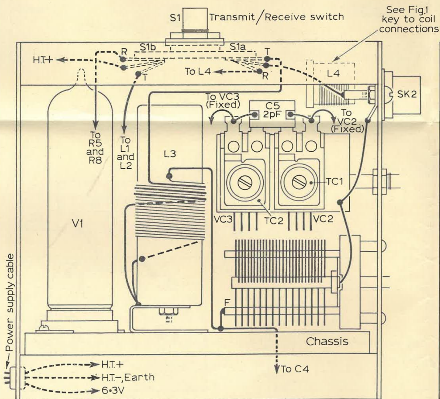
FIG. 4 SIDE VIEW OF TRANSCEIVER
