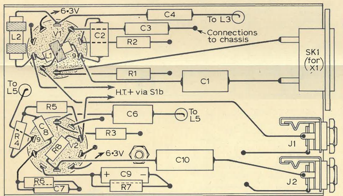
FIG. 3 UNDERSIDE VIEW OF CHASSIS
