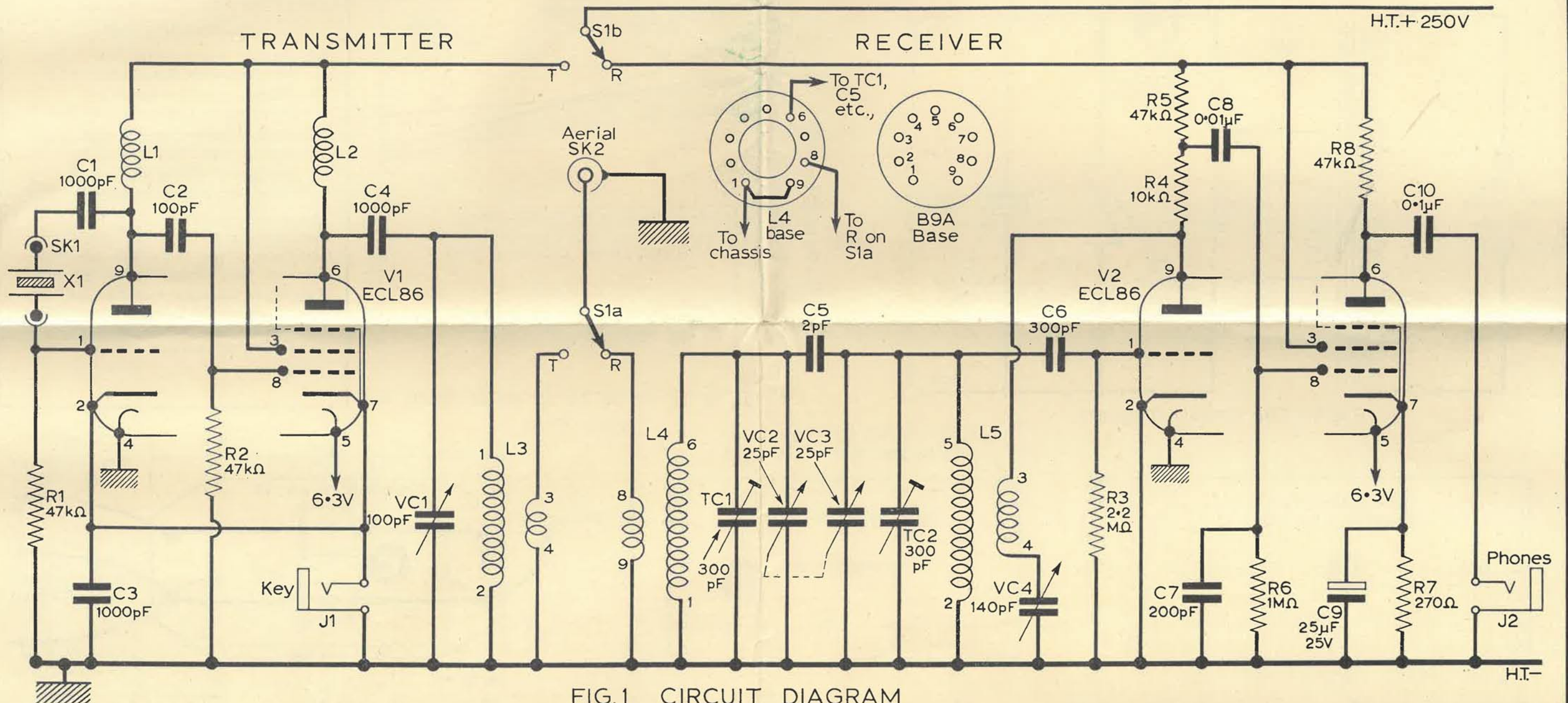
FIG. 1 CIRCUIT DIAGRAM
