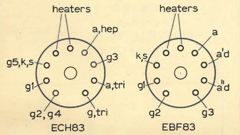
Fig. 7 VALVE BASES
