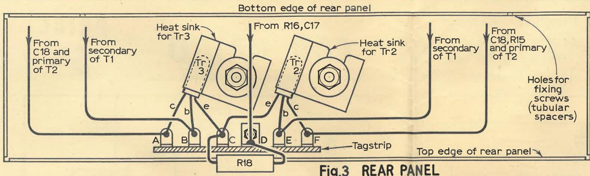
Fig. 3 REAR PANEL
