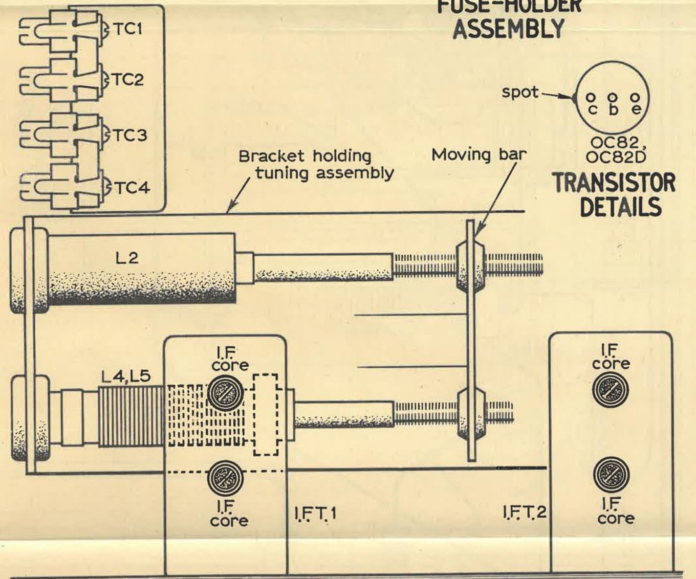
Fig. 9 ALIGNMENT DIAGRAM
