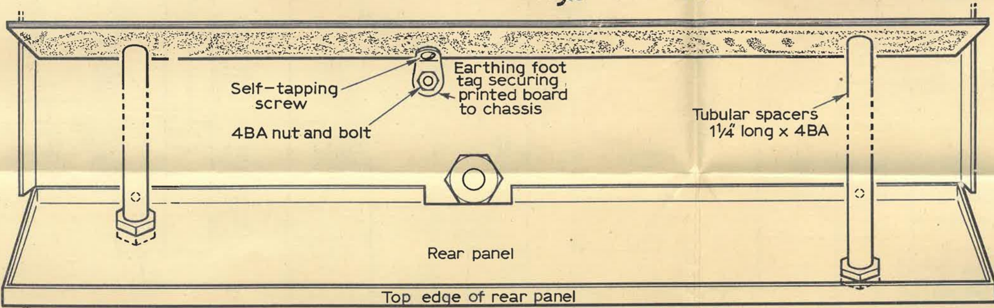
Fig. 4 SECURING PRINTED CIRCUIT BOARD
