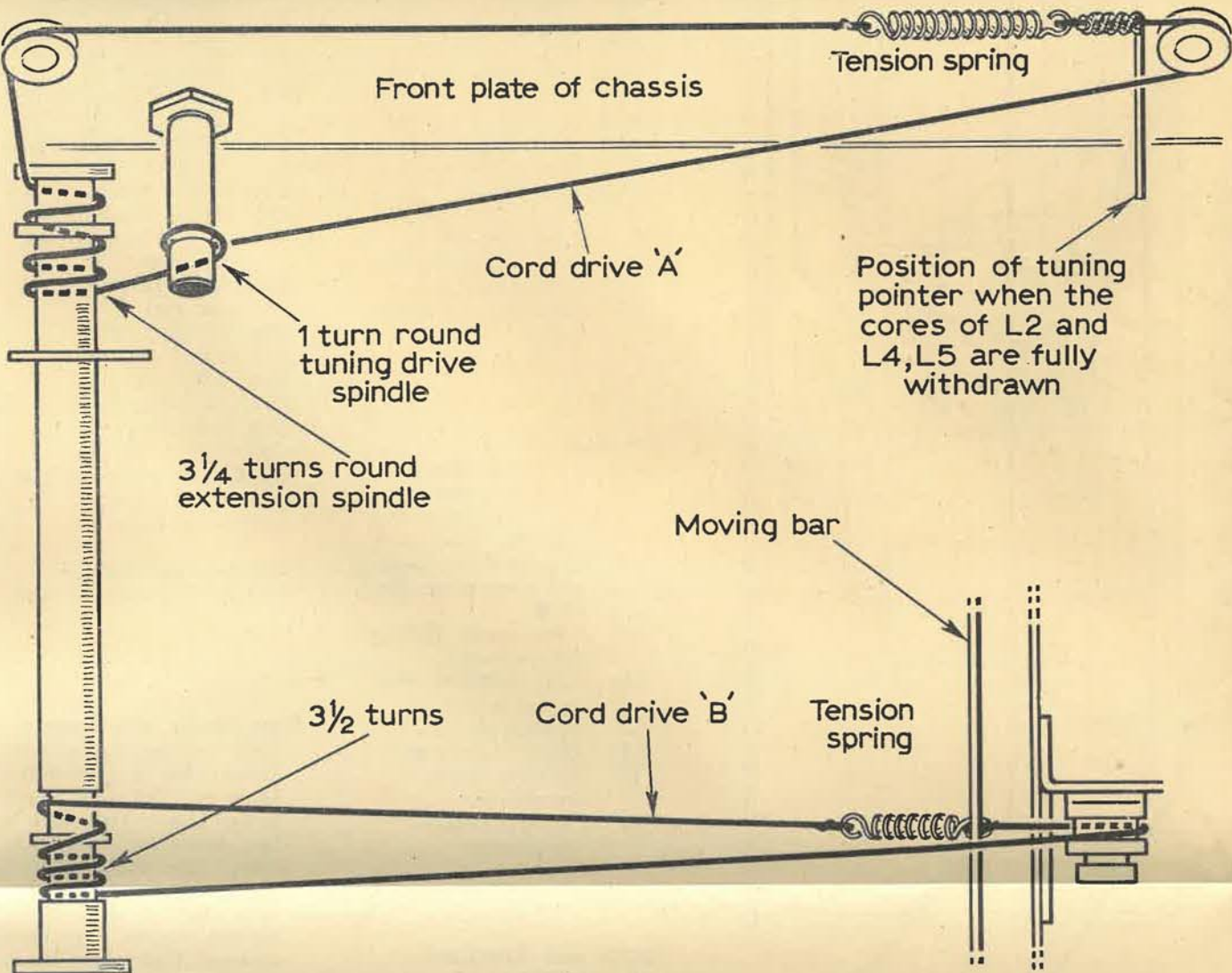
Fig. 6 CORD DRIVE DETAILS
