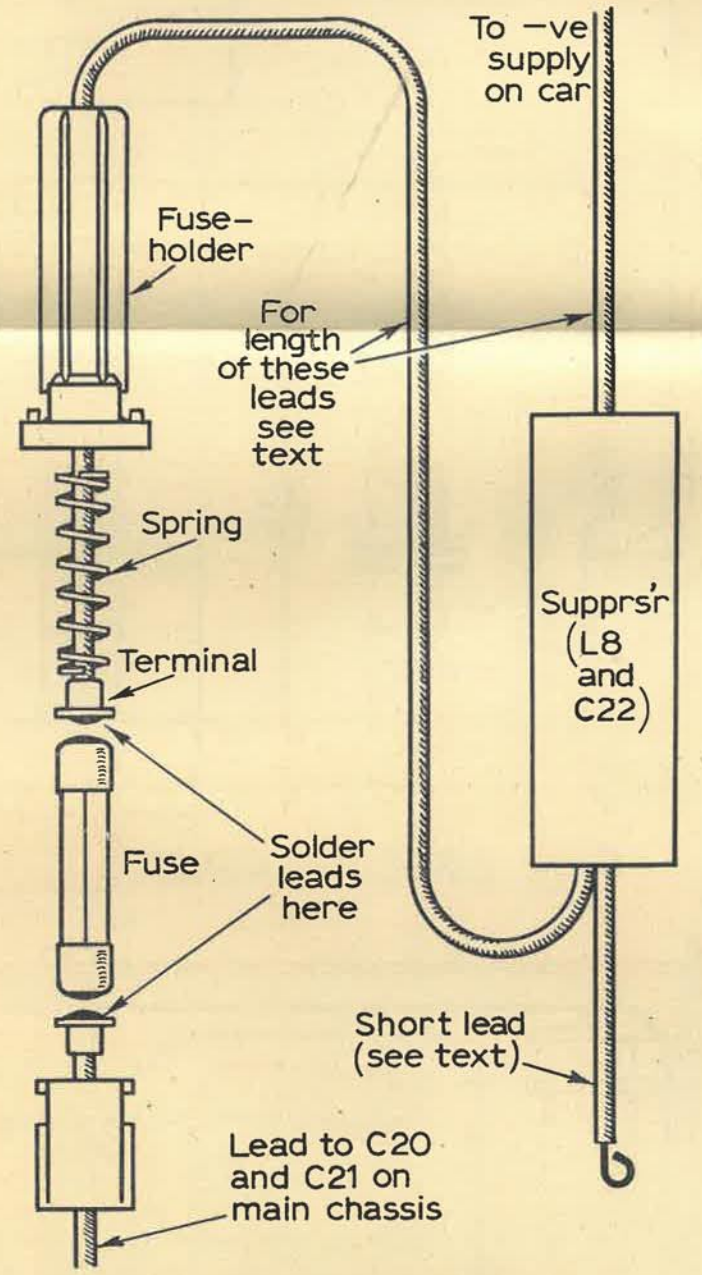
Fig. 8 SUPPRESSOR AND FUSE-HOLDER ASSEMBLY
