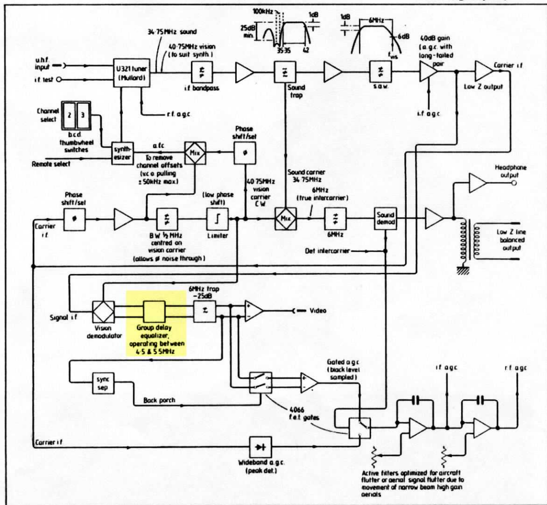
Fig. 97. Block diagram of the BBC-designed u.h.f. tv receiver, RC1/511, giving outputs of 1 volt composite video and good quality sound.
