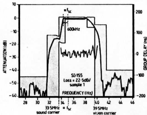
Fig. 96. Amplitude and group delay performance of u.a.w. filter recently introduced by Signal Technology.
