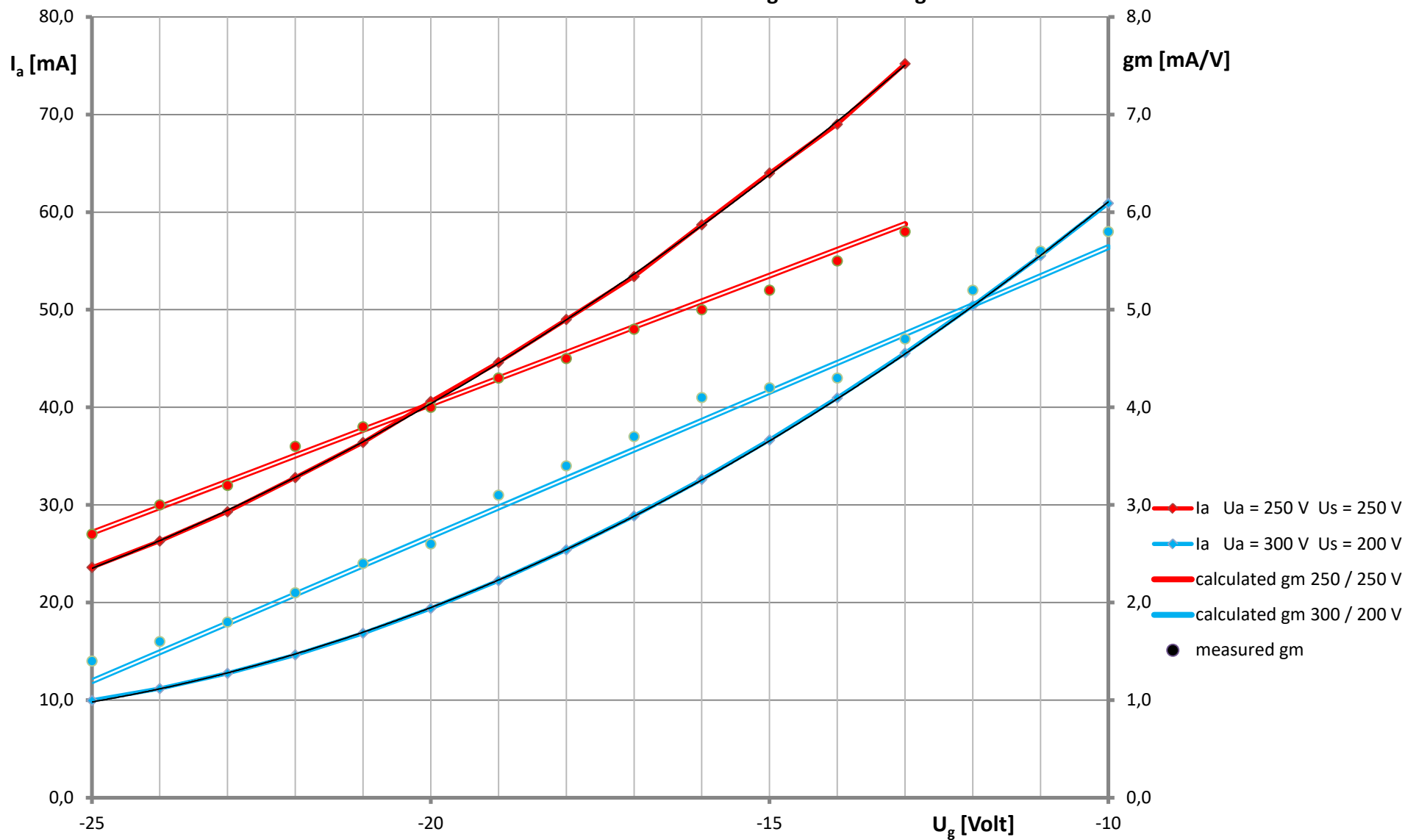
6L6 valve characteristics I_a=f(U_g) ; gm=f(U_g) (Russian made bogie valve from Kurt Schmid)
