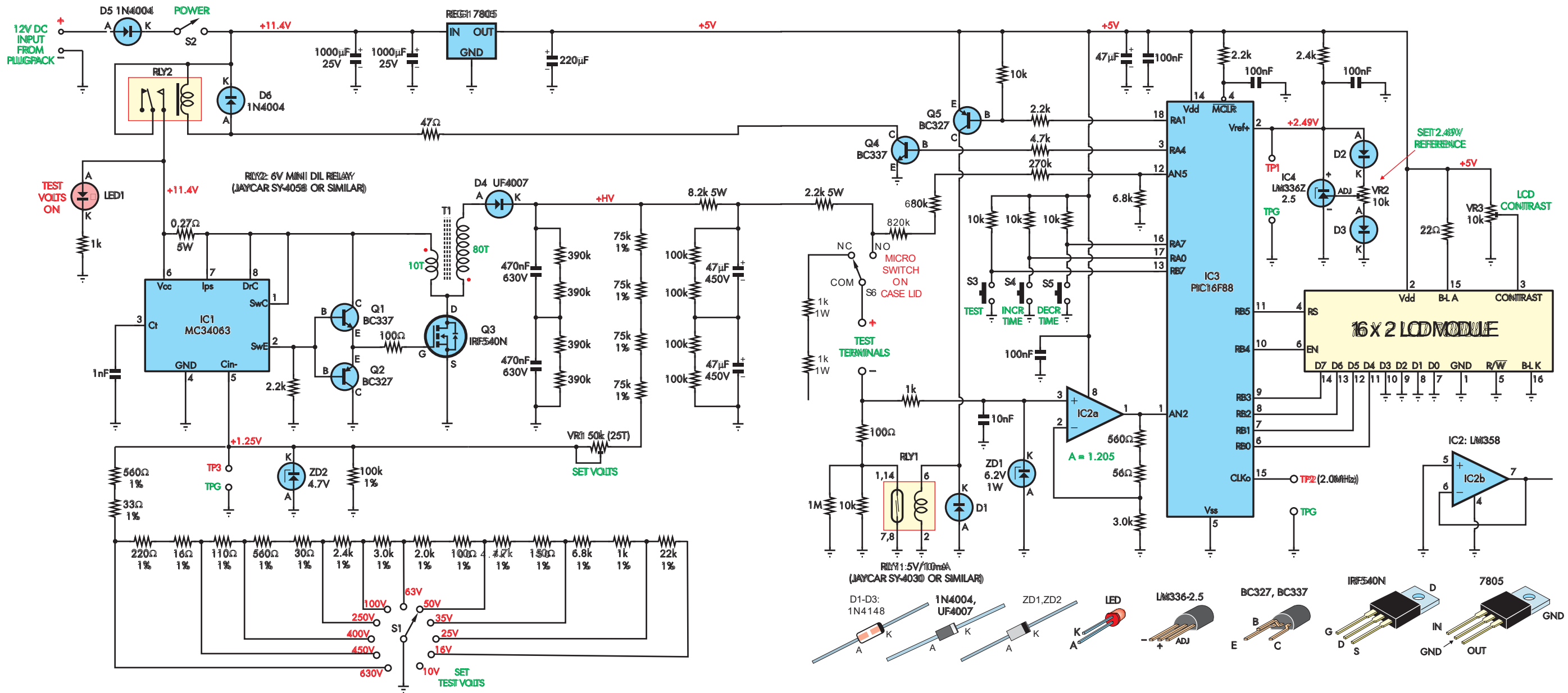
ELECTROLYTIC CAPACITOR REFORMER AND TESTER
